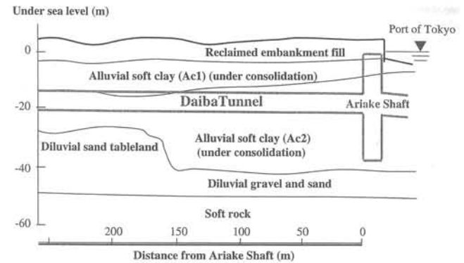
Figure 3. Soil profile and location of the tunnel.
