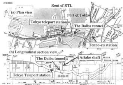
Figure 1. The layout of the Daiba Tunnel.
