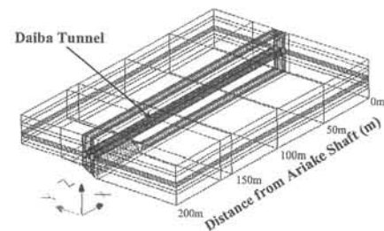
Figure 8. Finite element meshes.
