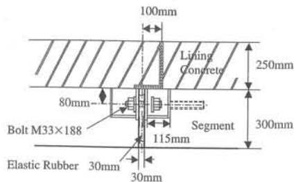
Figure 6. Expansion joint system.
