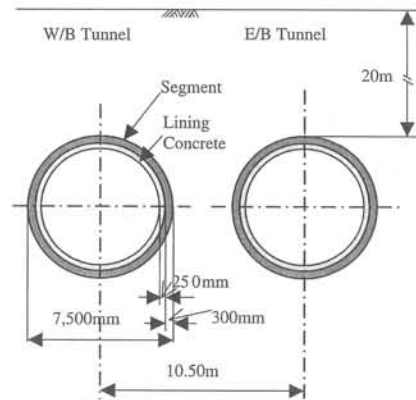
Figure 2. Cross section of the Daiba Tunnel.
