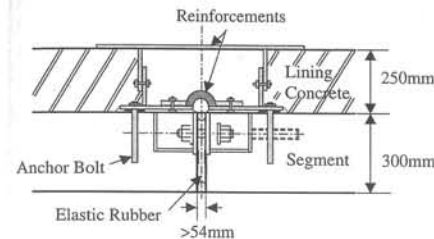
Figure 7. Reinforcement of expansion joint.
