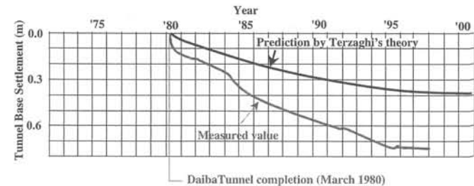
Figure 4. Settlement at Daiba Eastbound Tunnel base where the section is 70 metres away from Ariake Shaft.
