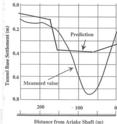
Figure 5. Longitudinal displacement of tunnel.
