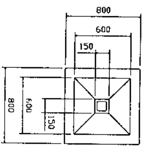
FOOTING COLUMN (Scale 1:40)
