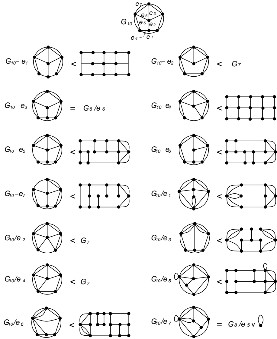
Fig. 11. G_{10} - e_i, G_{10}/e_i .
