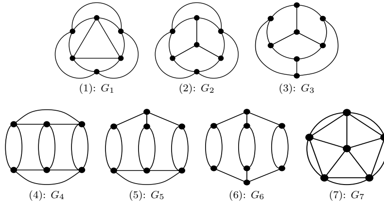
Fig. 1. Previously known seven elements of \Omega(T) .
