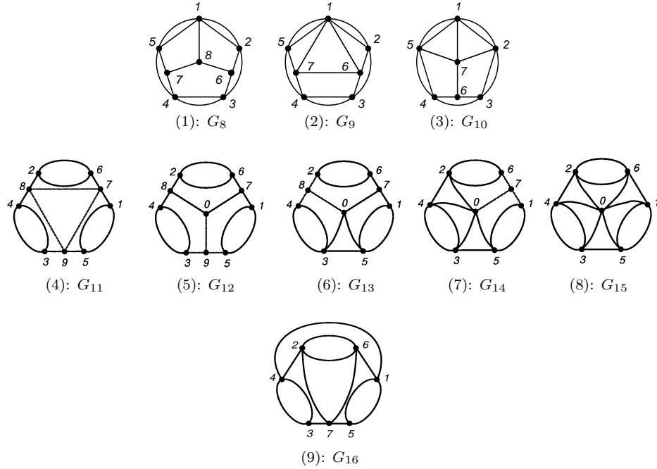
Fig. 4. Newly found forbidden graphs G_8, \dots, G_{16} .
