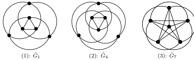
Fig. 2. Knotted projections of G_1 , G_4 and G_7 .
