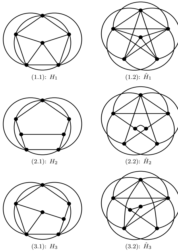
Fig. 6. A major H_i of the eye-graph and its knotted projection \hat{H}_i .
