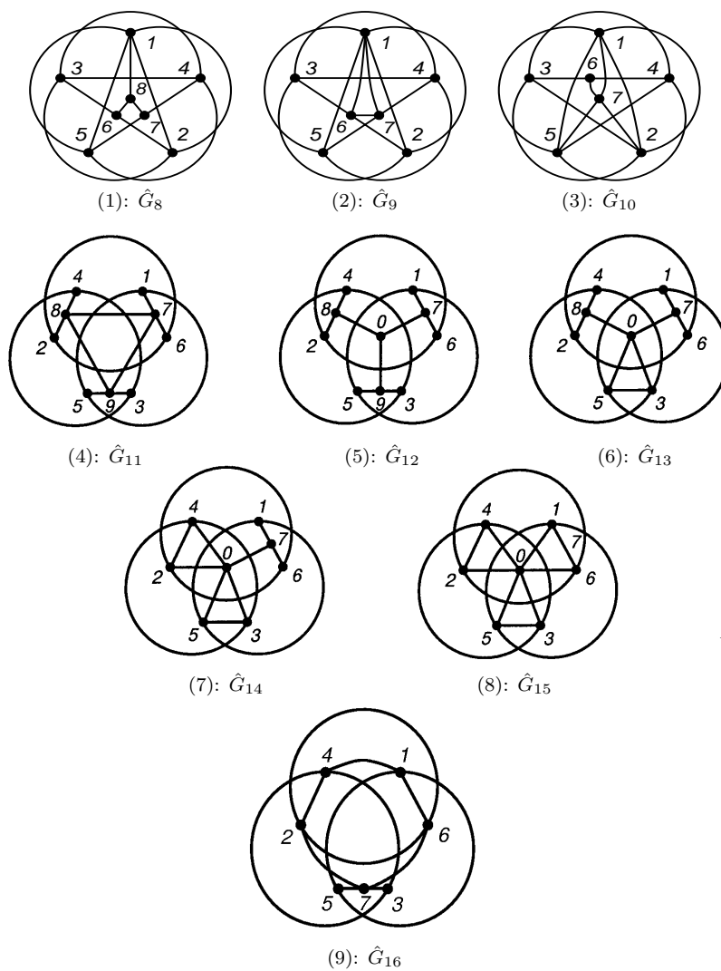
Fig. 5. Knotted projections of G_8, \dots, G_{16} .
