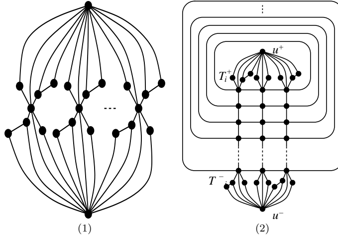
Fig. 3. A bi-focal and a three-line web.
